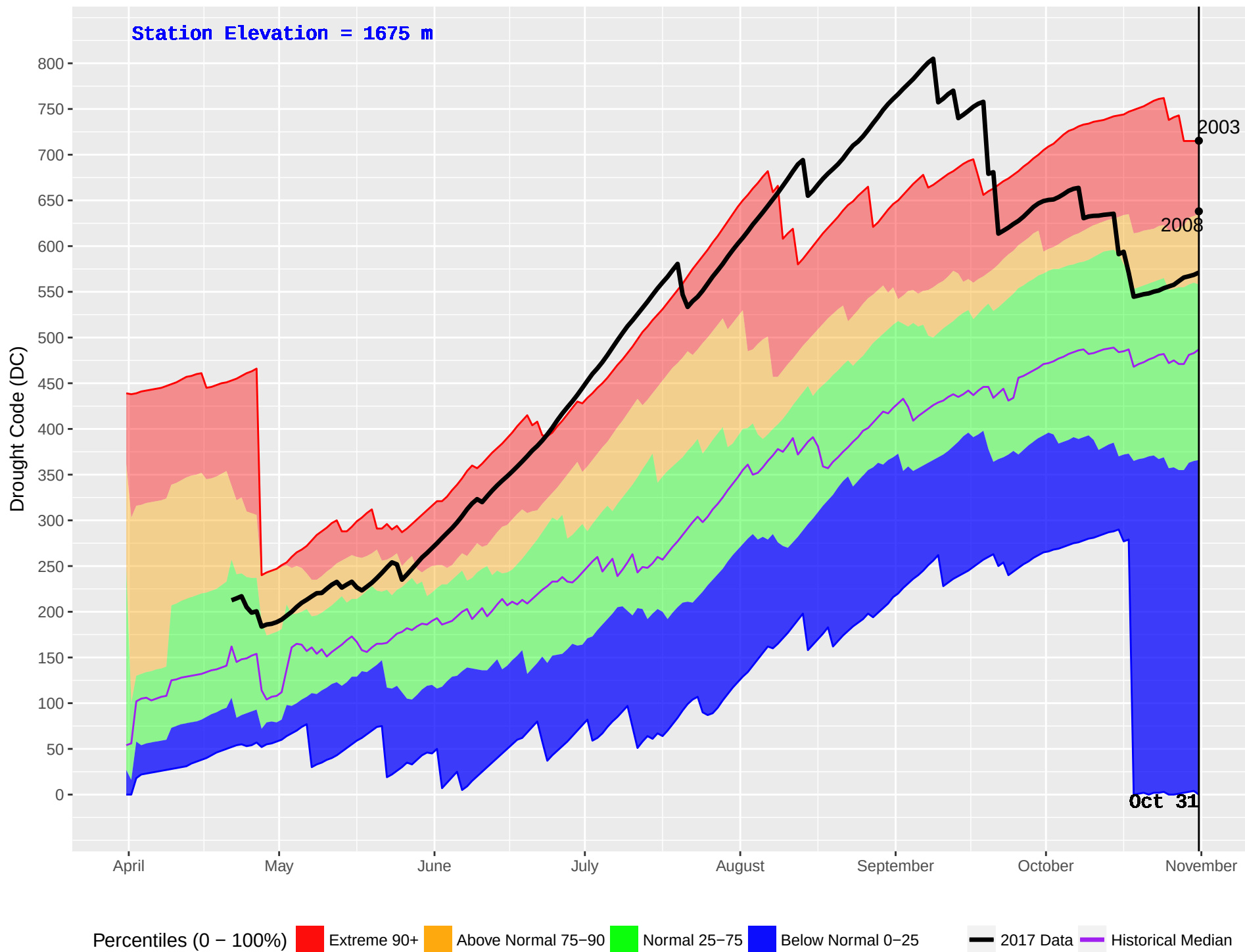
GASPARD (222) : Historical (1992–2016) and Current (2017) Noon Drought Code (DC)
