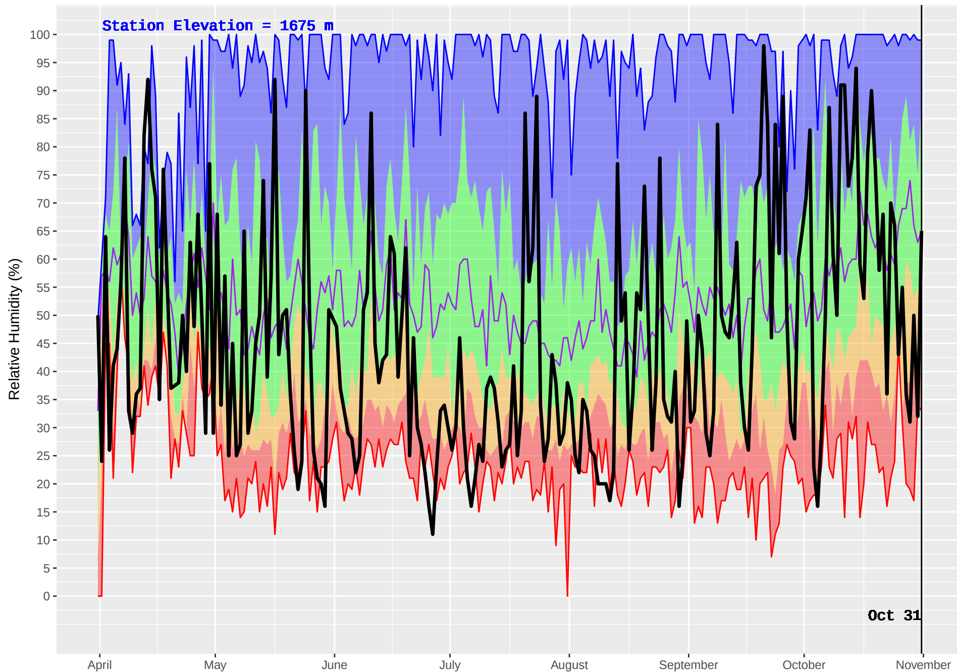
GASPARD (222) : Historical (1992–2016) and Current (2017) Noon Relative Humidity
